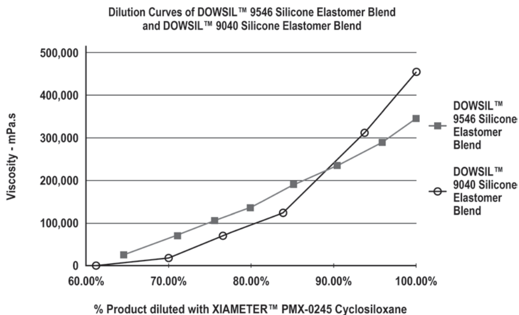
Figure 2: Rheological flow comparison of DOWSIL 9546 Silicone Elastomer Blend and DOWSIL 9040 Silicone Elastomer Blend.
